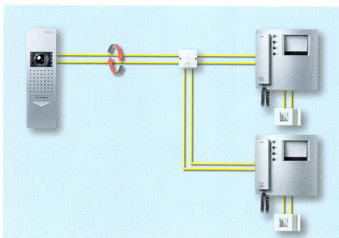
Video-Set VSS 711-0 extended by a second internal video station (in-house telephone/monitor combination) VIS 711-0. An additional video extension box VEB 711-0 and a second line rectifier VSNG 711-0 are required for connection. Functional characteristics: Parallel operation of the in-house telephone/monitor combination, i.e. a door call with picture connection is transmitted to both in-house telephone/monitor combinations. The call is accepted by lifting the receiver.
